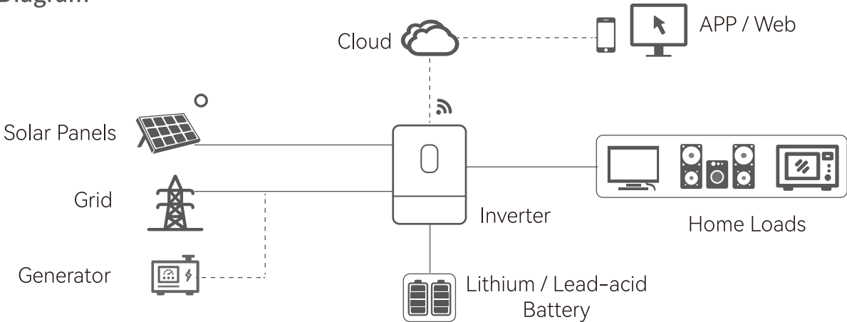
System Diagram
